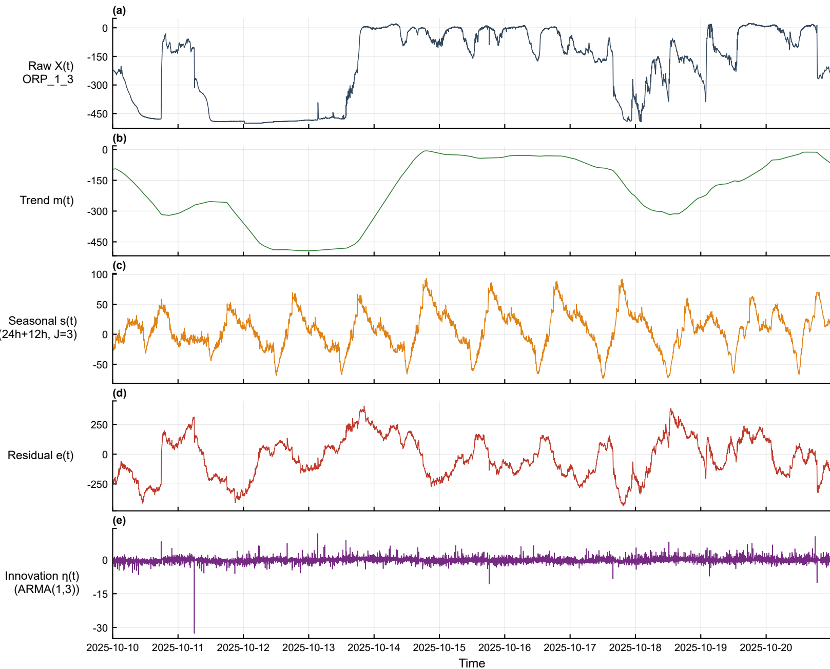
Multi-scale decomposition — ORP_1_3 (pre_anoxic_rear, min) [2025-10-10~2025-10-20]
